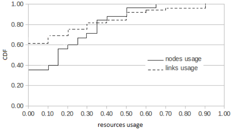
Figure 3: CDF for resource usage in experiment C3
