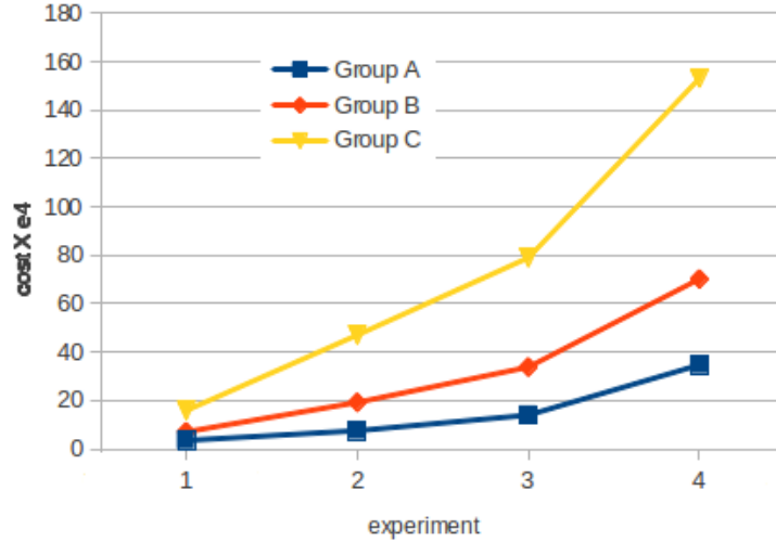
Figure 2: Mapping cost
