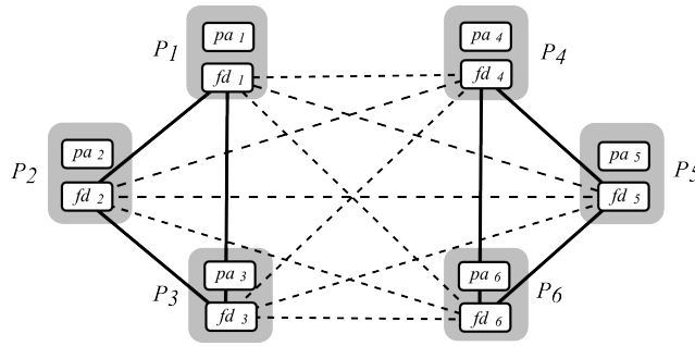
Figure 1: Application topology with failure detector \mathcal{P}
