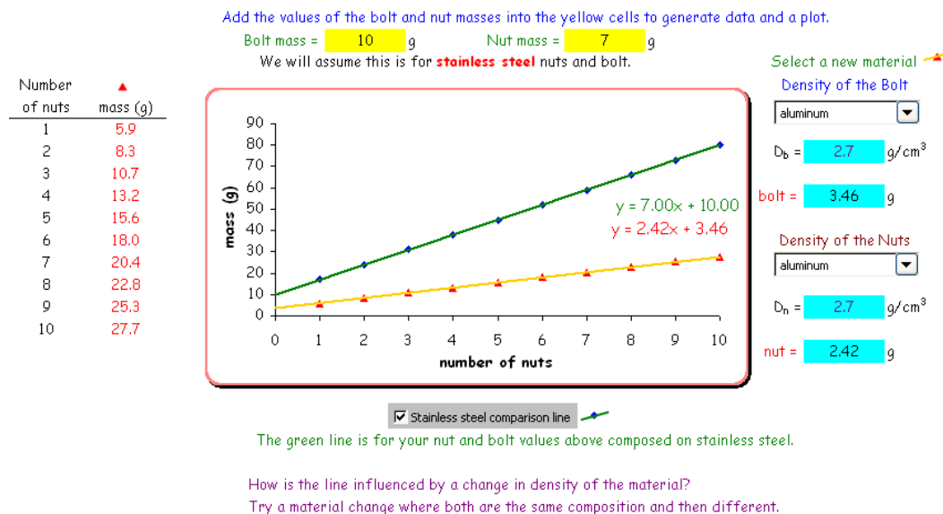
Figure 4. Material Density Tab – Compares Aluminum to Stainless Steel
